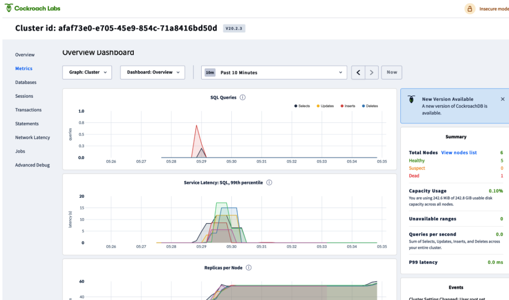
Figure 5.6 – Metrics dashboard
